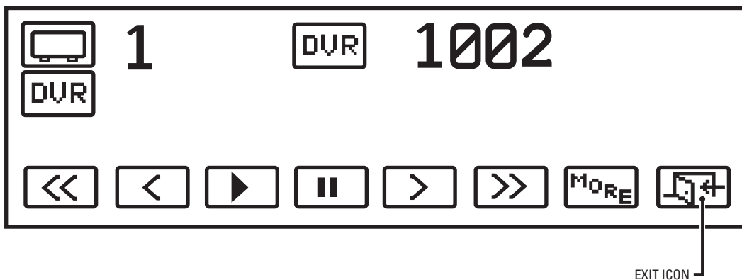
Figure 47. DVR Menu 1
